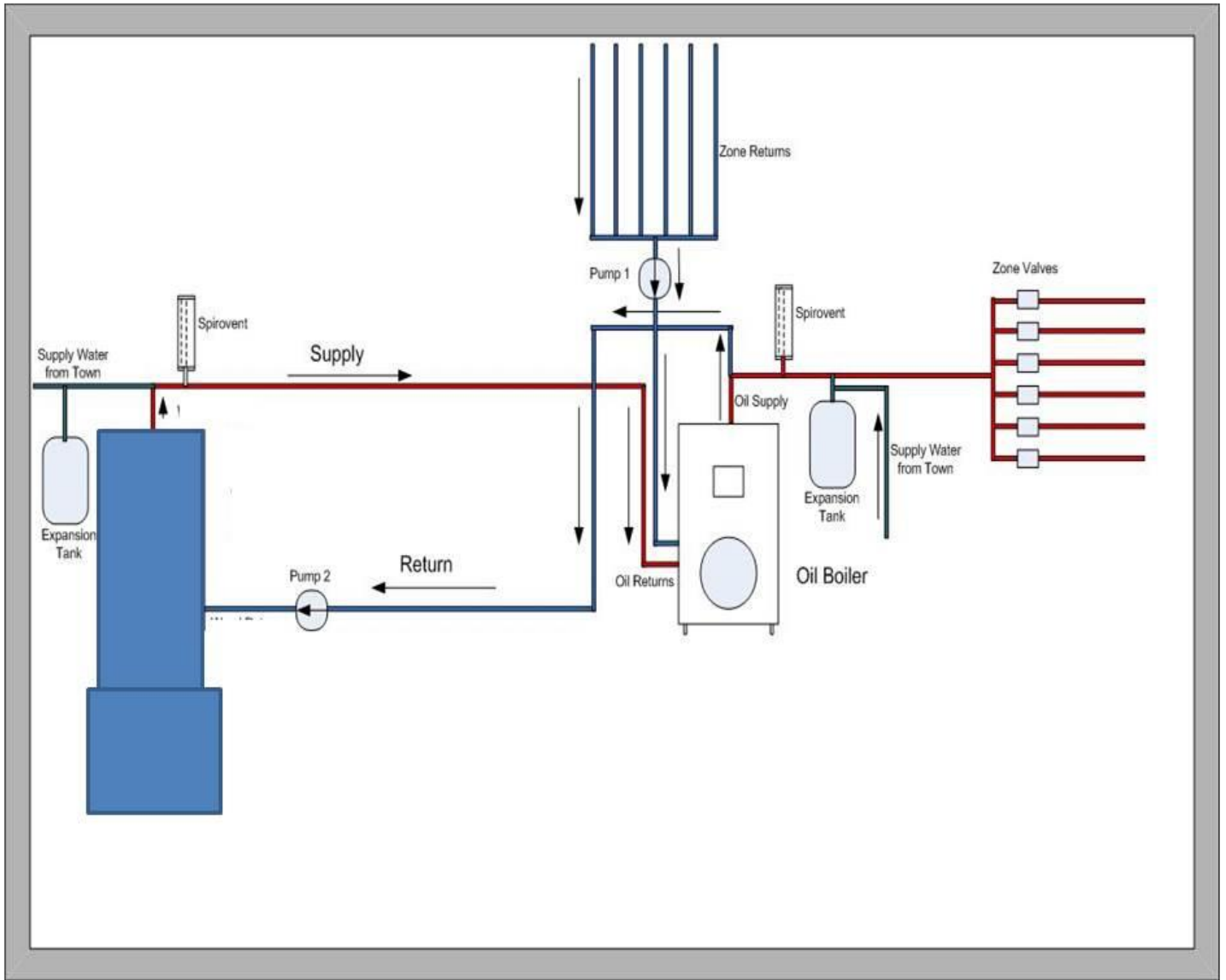
Typical Dual Boiler Installation (for reference only)
