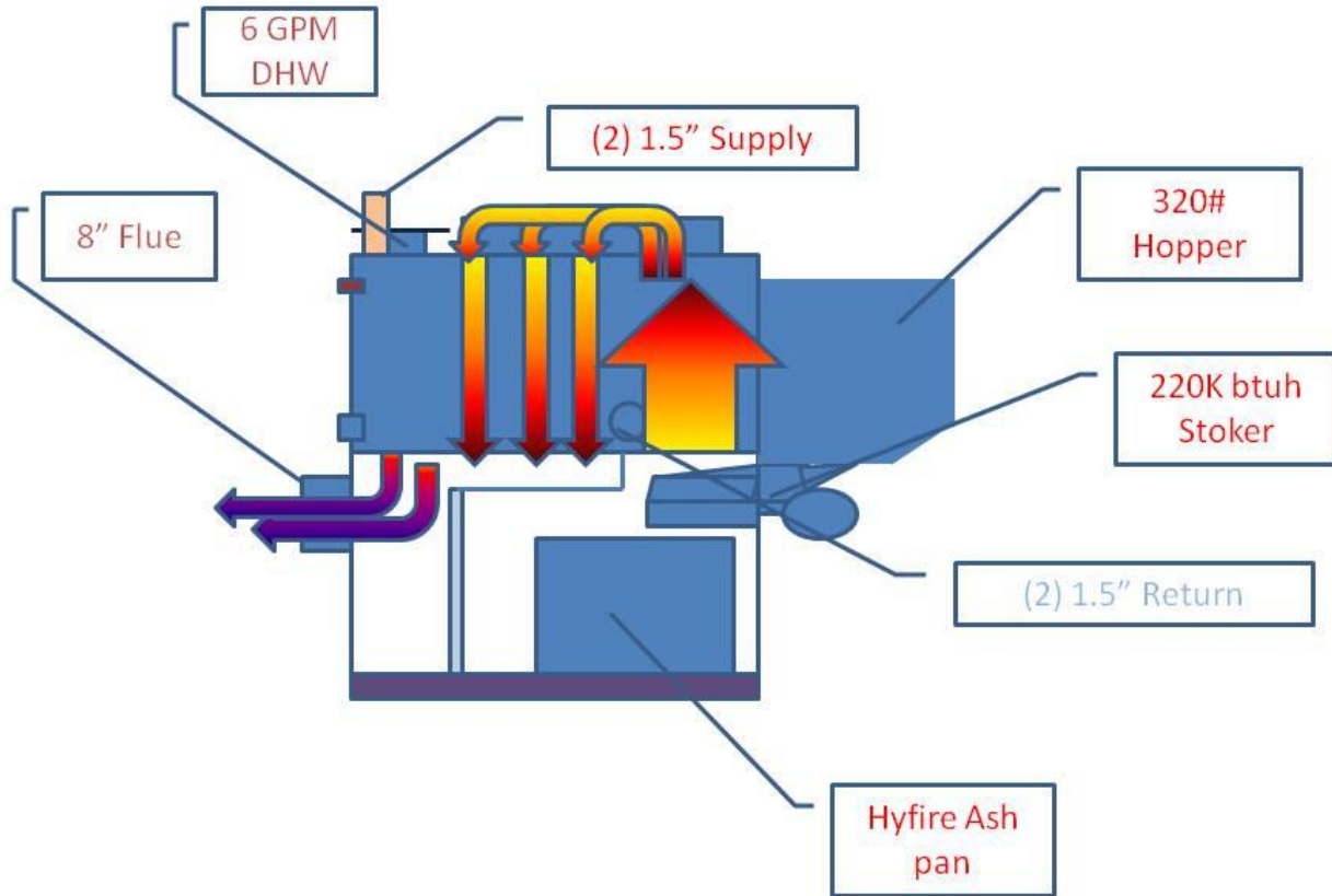
Leisure Line 220 Boiler (Axeman Anderson Pressure Vessel)
